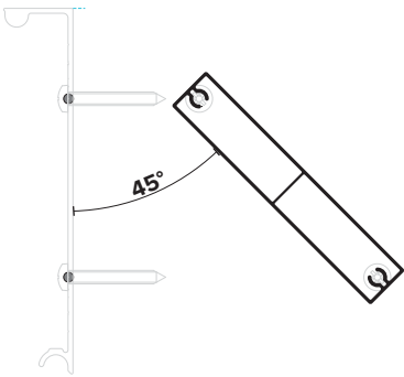
VERTICAL SECTION WITH INCLINATION 45°
