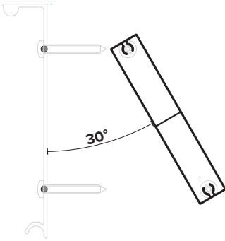
VERTICAL SECTION WITH INCLINATION 30°
